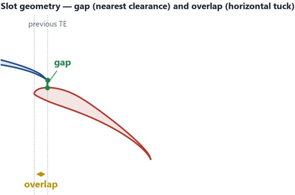
Figure 2 — Slot definitions on a real placement. Gap is the smallest clearance from the previous trailing edge to the flap surface; overlap is the horizontal tuck of the flap nose under that trailing edge.
